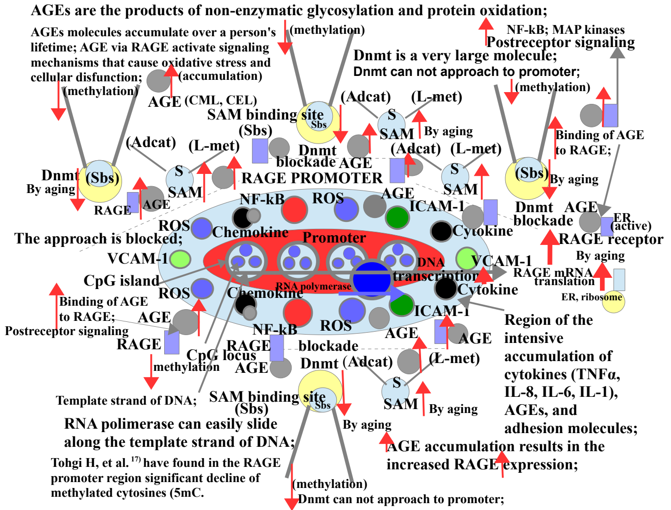
Fig.2. RAGE promoter-Dnmt and SAM can not approach to DNA
